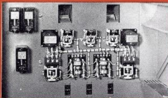
Power and overload relays are accessible from the front of the transmitter. A hinged cover encloses dust and provides personnel protection.
